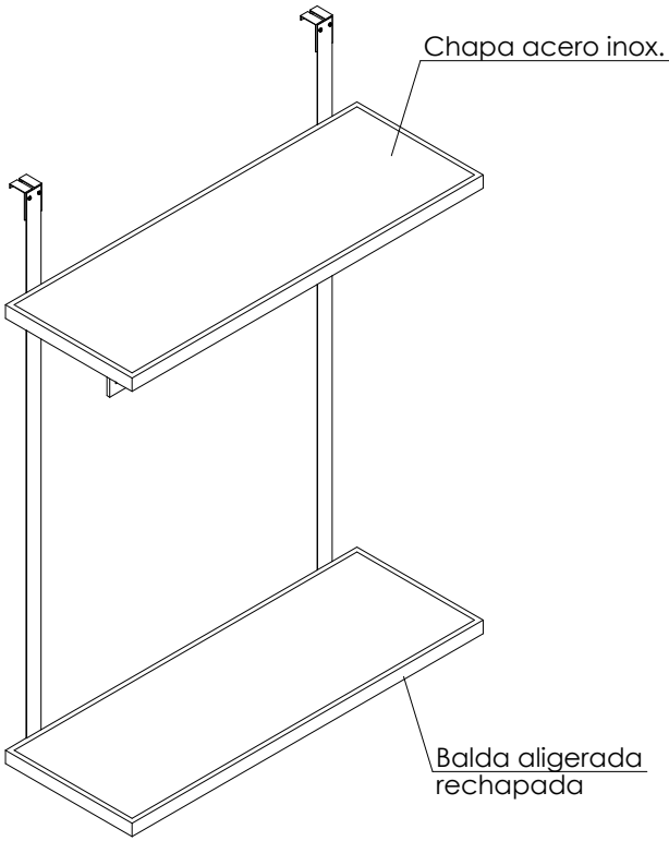
VISTA 3D
