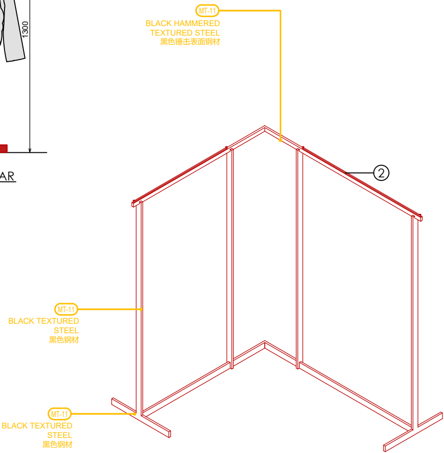
VISTA 3D
