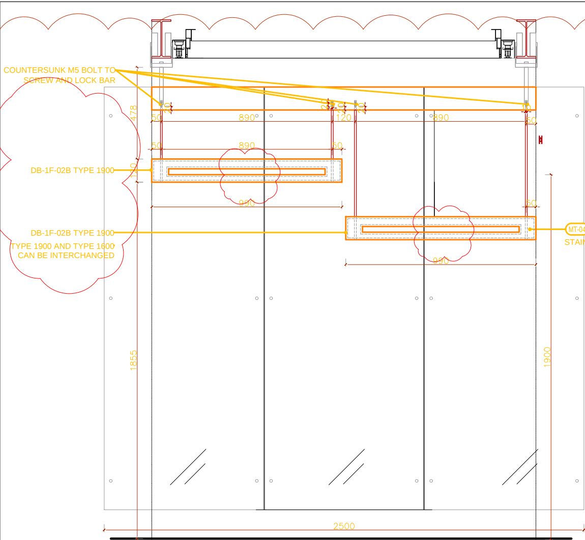
1 1:10 FRONT ELEVATION
