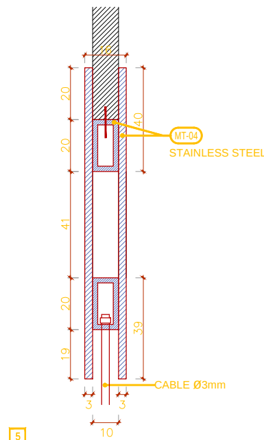
5 1:10 DETAIL
