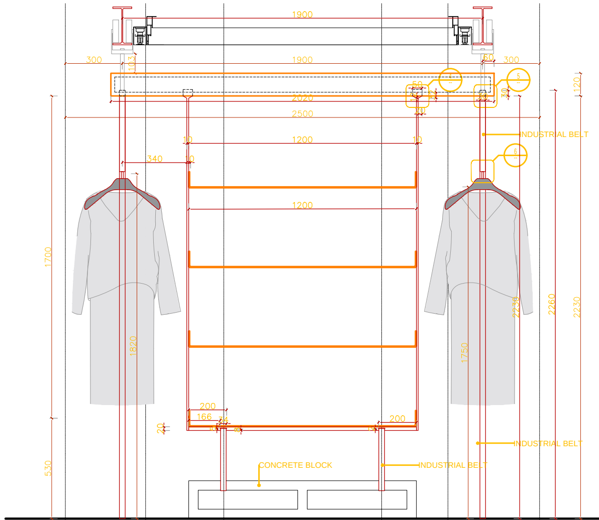
1 1:10 FRONT ELEVATION
