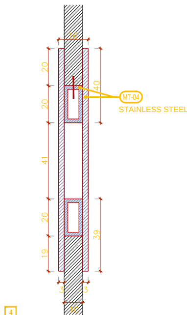
4 1:10 DETAIL
