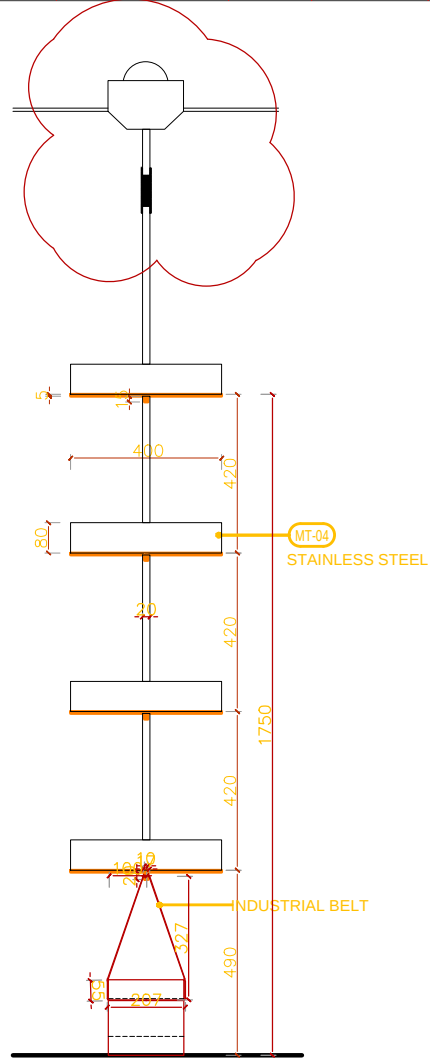
2 1:10 SECTION
