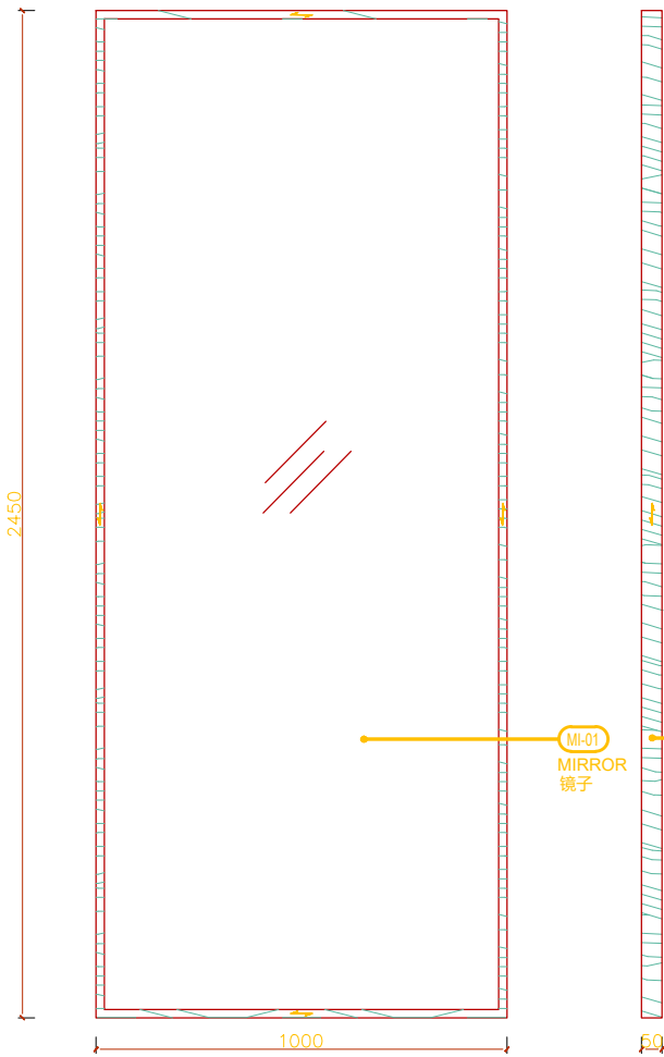
5 镜子正立面 1:10 MIRROR FRONT ELEVATION
