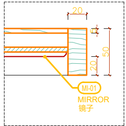
7 镜子细节 1:10 MIRROR DETAIL
