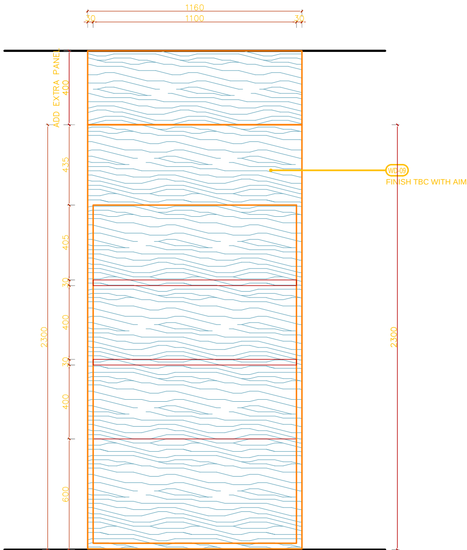
2 1:10 FRONT ELEVATION
