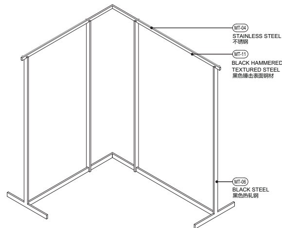
VISTA 3D
