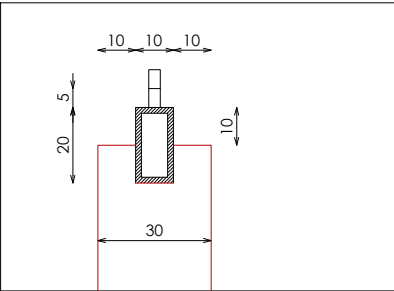
DETALLE A FOLLOW ZARA STANDARDS
