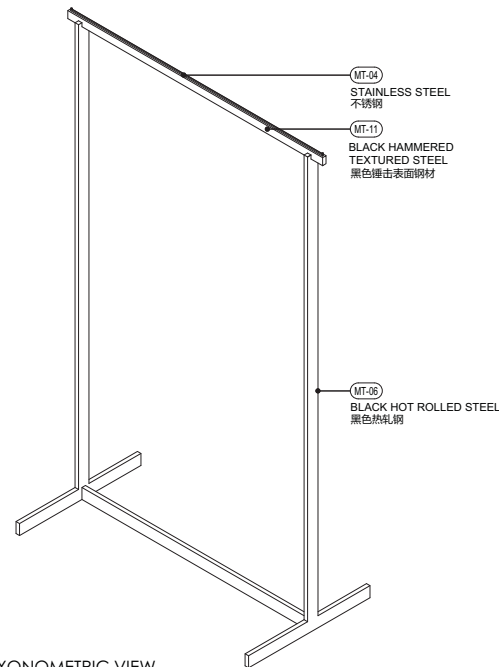
AXONOMETRIC VIEW
