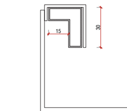
5 节点 1:1 DETAIL COMPLEMENTS
