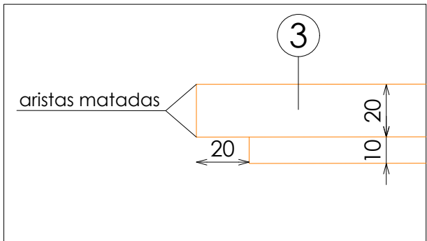
DETALLE TARIMA
