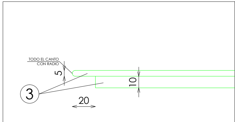
DETALLE TARIMA
