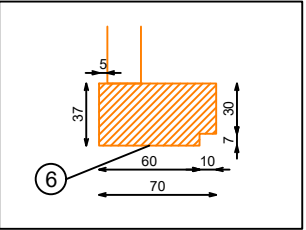
DETALLE REMATE DER.
