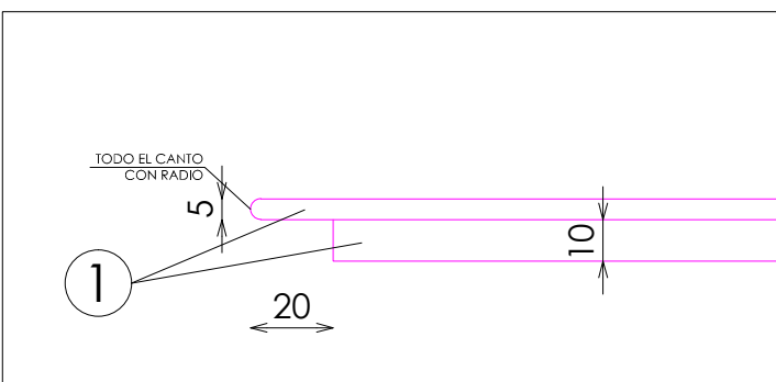
DETALLE TARIMA
