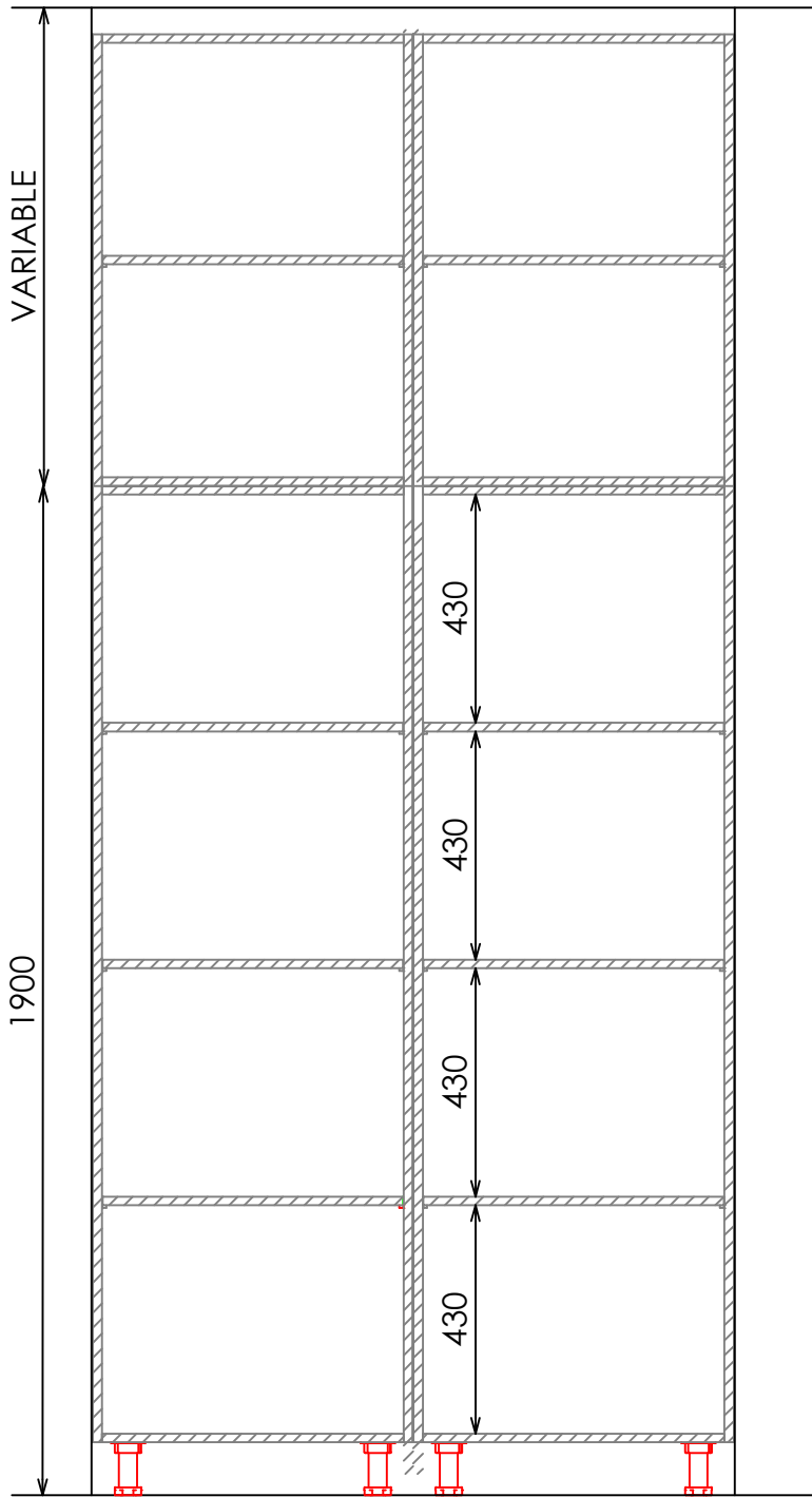
ALZADO INTERIOR
