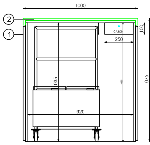
ALZADO INTERIOR
