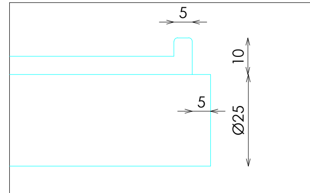
DETALLE TARIMA
