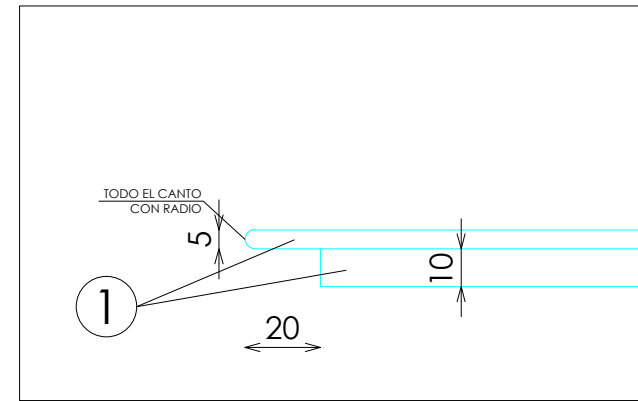
DETALLE TARIMA
