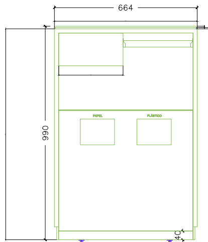
ALZADO FRONTAL ELEVATION
