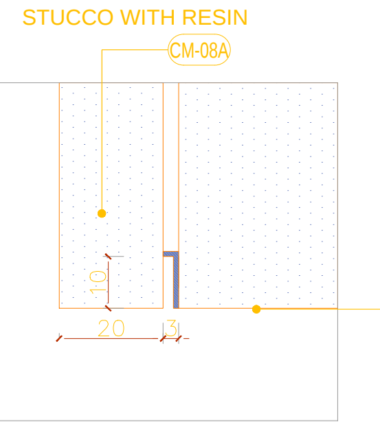
6 1:10 DETAIL
