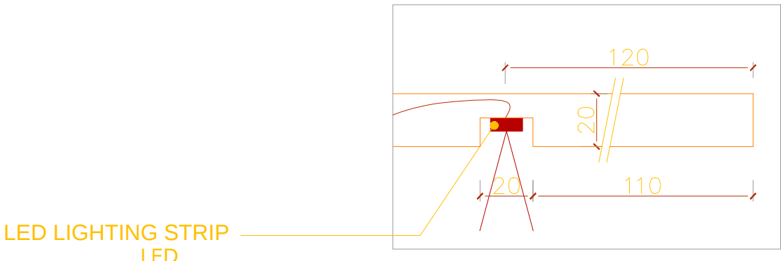
4 1:5 DETAIL
