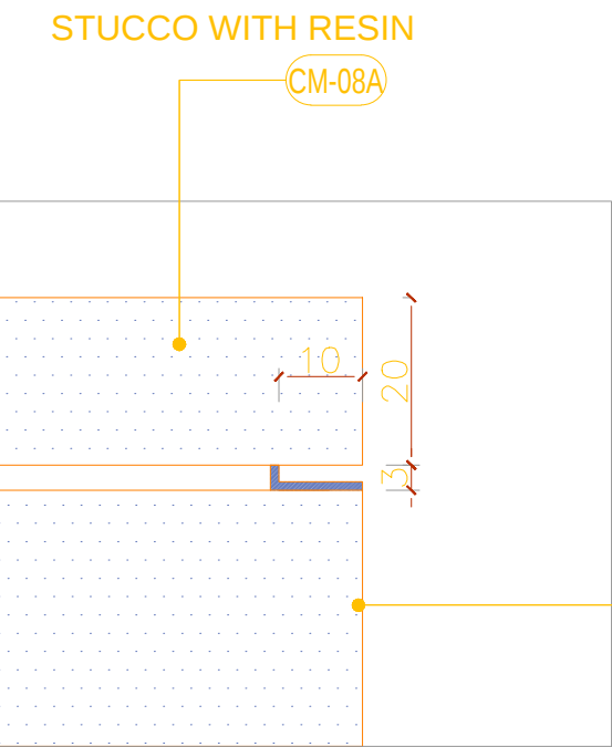
5 1:10 DETAIL
