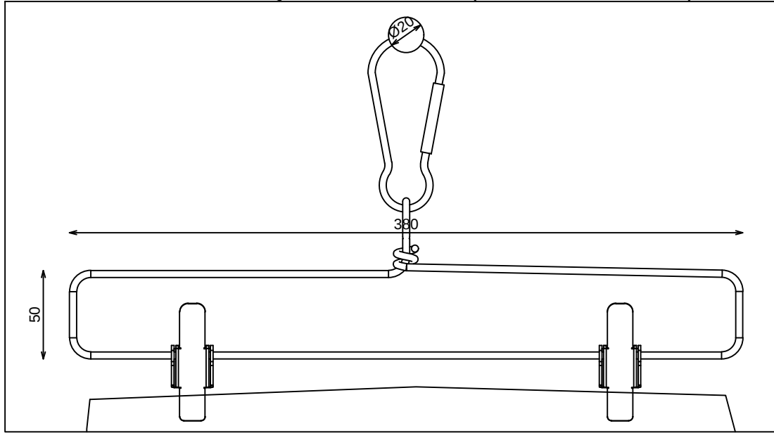
DETALLE PERCHA (FORMAS INOXMAN)
