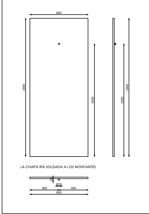
DETALLE PANEL
