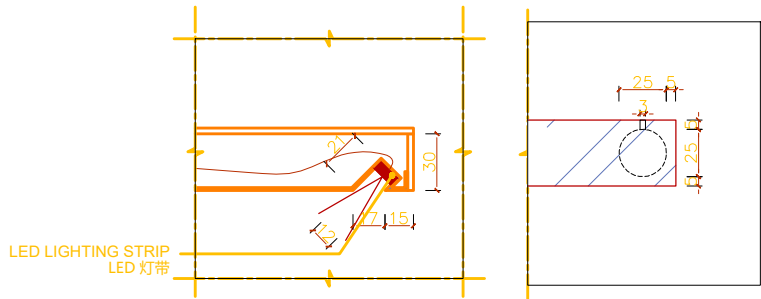
6:12 节点 DETAIL
