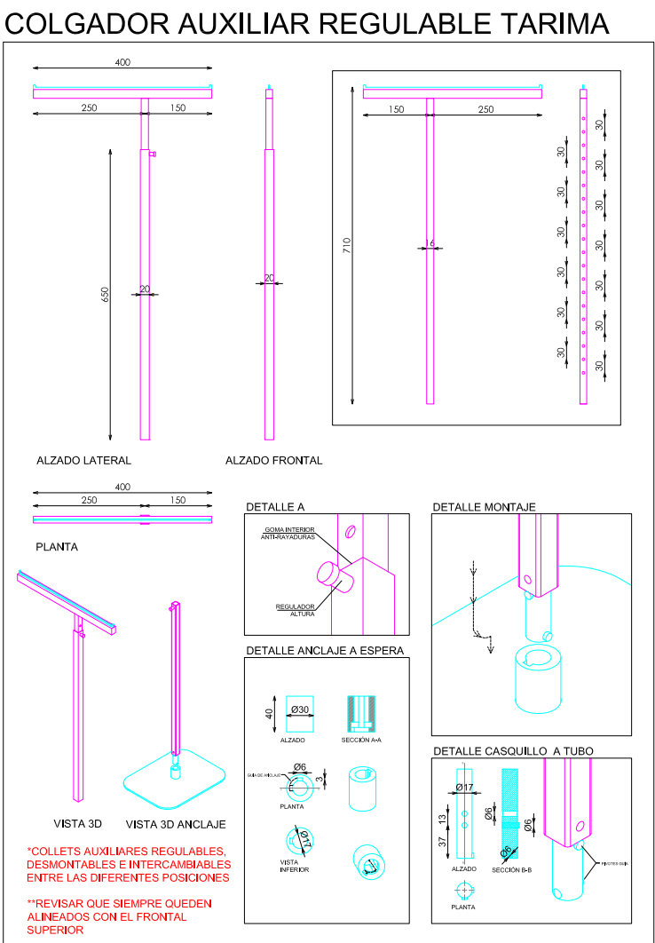
COLGADOR AUXILIAR REGULABLE TARIMA
