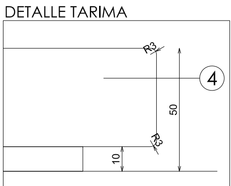
DETALLE TARIMA
