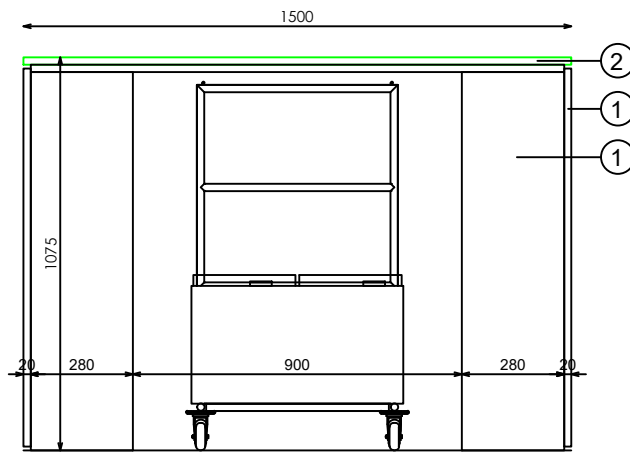
ALZADO INTERIOR
