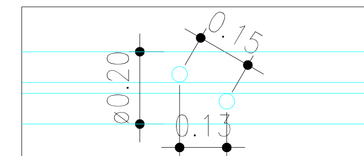
DETALLE TARIMA
