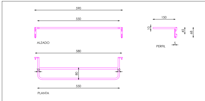
DETALLE TARIMA
