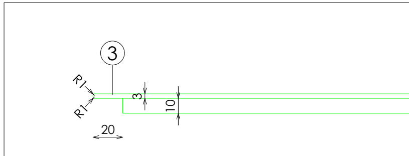
DETALLE TARIMA
