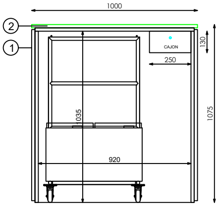
ALZADO INTERIOR
