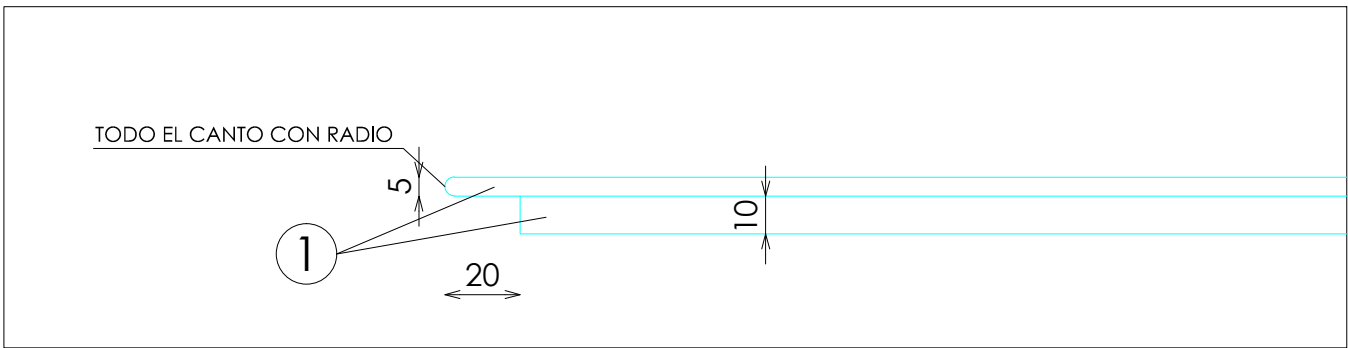
DETALLE TARIMA
