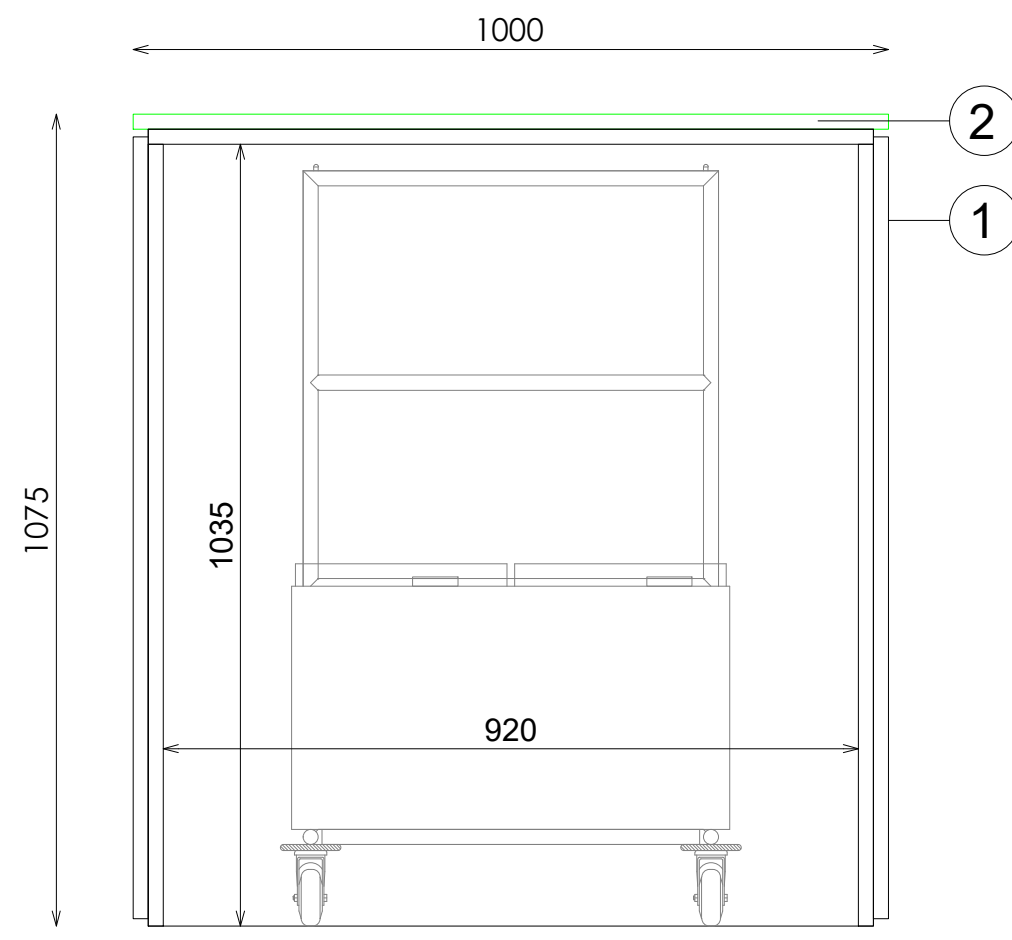
ALZADO INTERIOR
