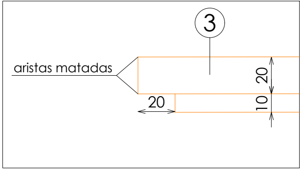
DETALLE TARIMA
