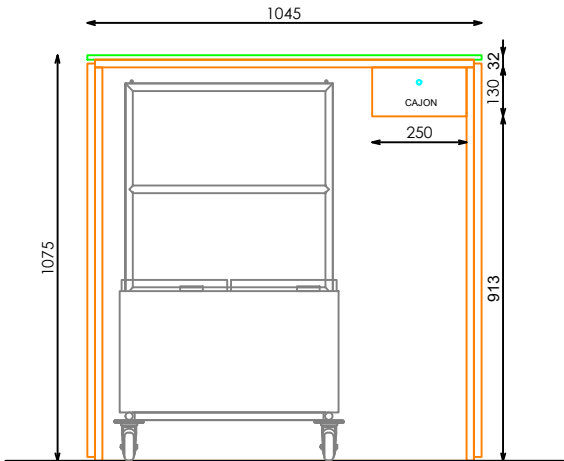
ALZADO INTERIOR
