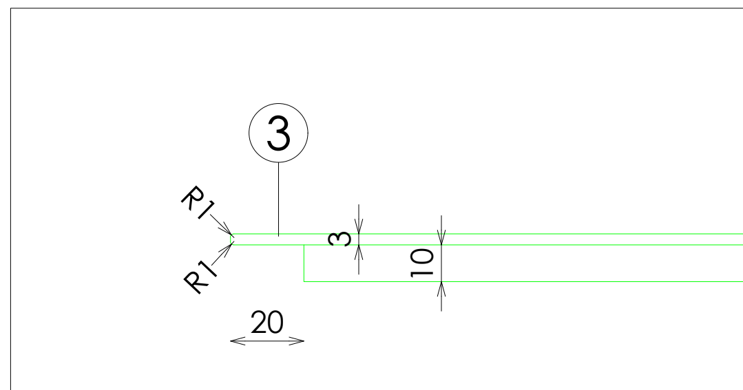
DETALLE TARIMA
