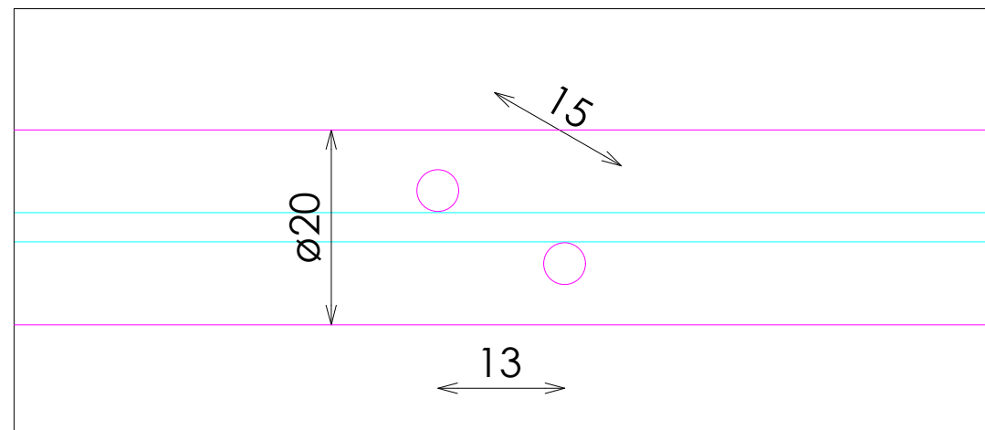
DETALLE TARIMA
