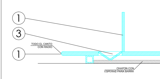
DETALLE BASE
