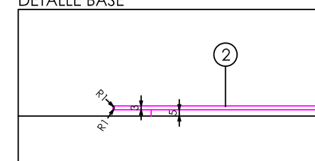
DETALLE BASE
