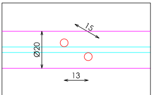
DETALLE TARIMA
