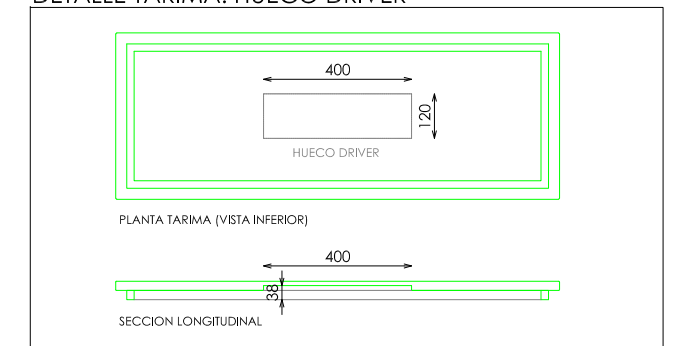
DETALLE BASE
