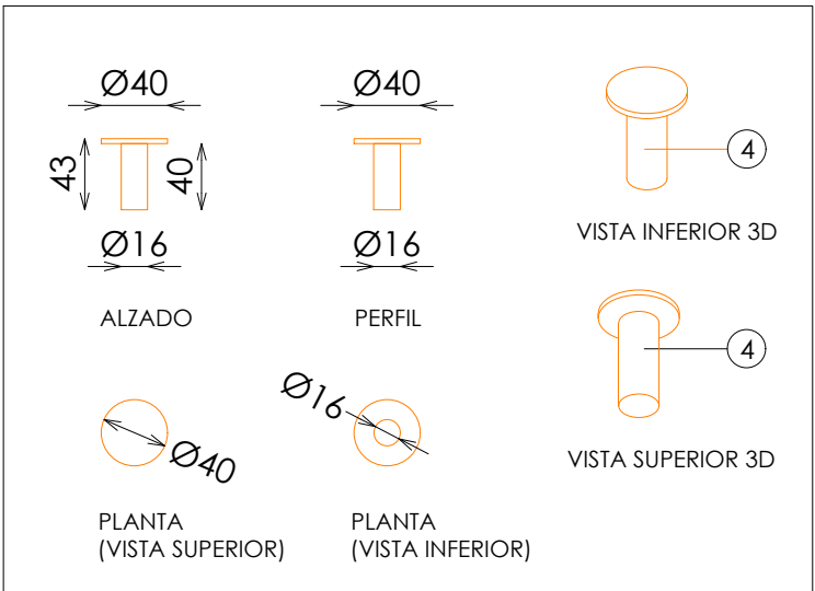
DETALLE BASE
