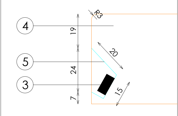
DETALLE BASE
