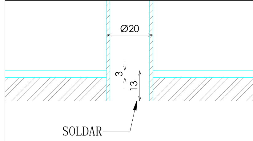
DETALLE TARIMA
