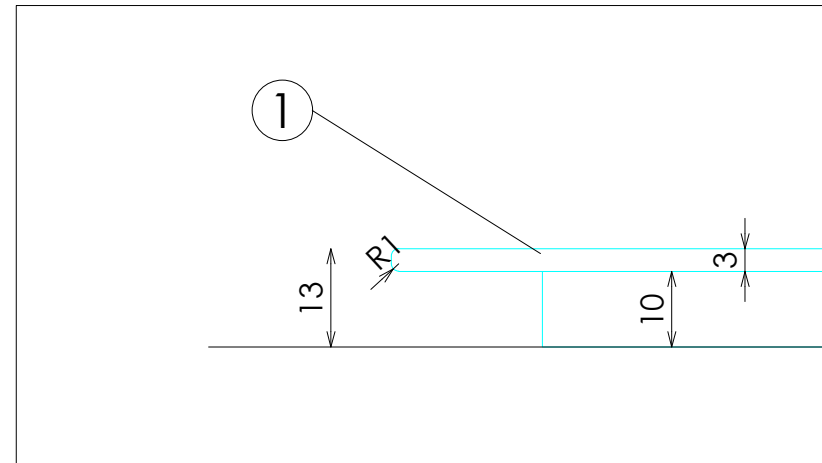
DETALLE TARIMA
