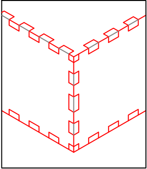
DETALLE UNION
