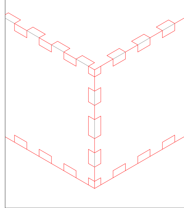
DETALLE UNION
