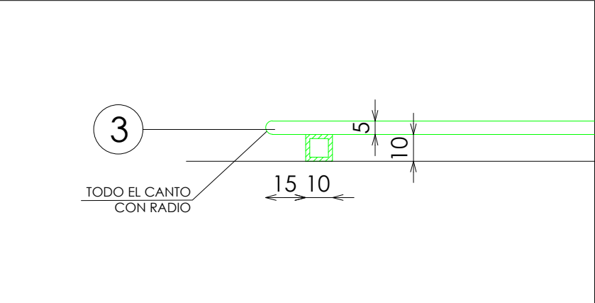
DETALLE BASE
