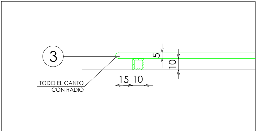
DETALLE BASE
