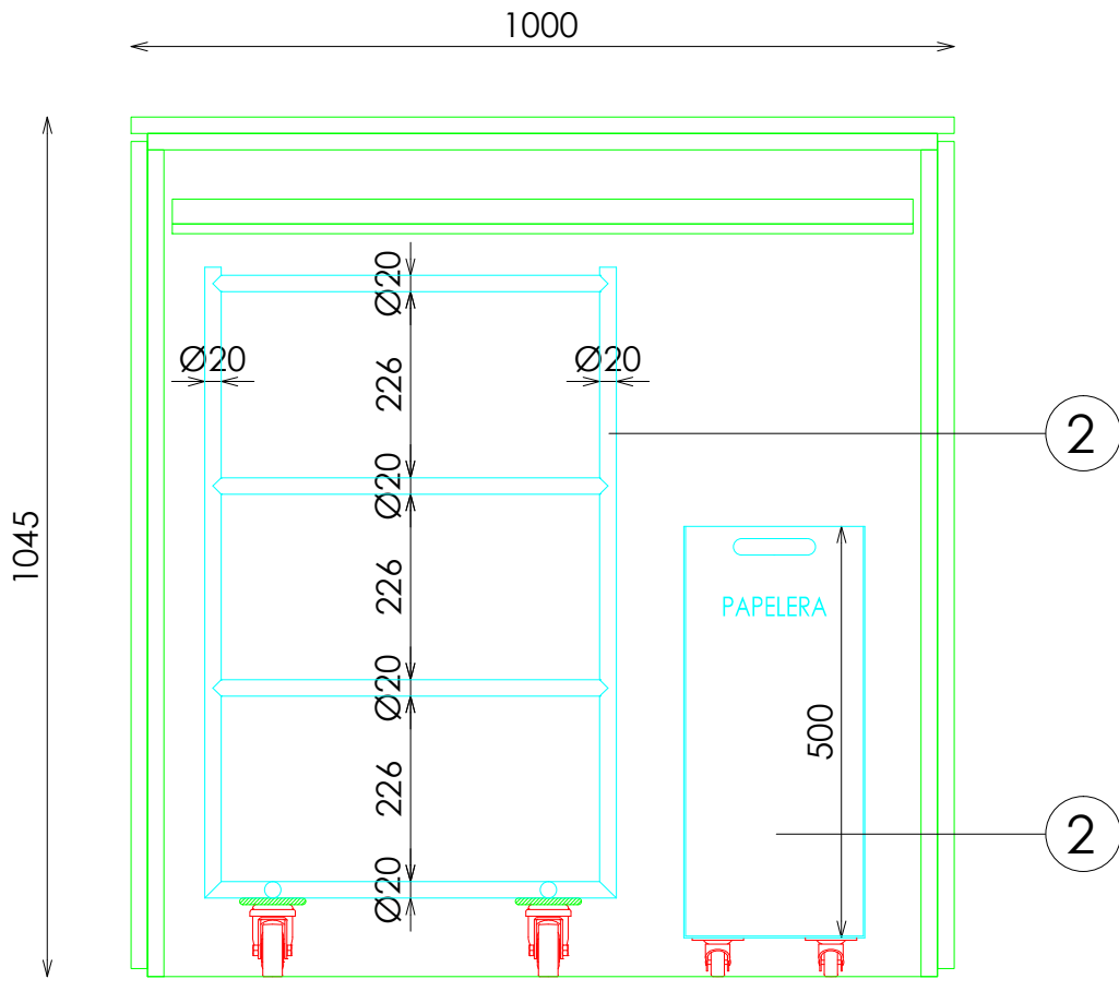
ALZADO INTERIOR
