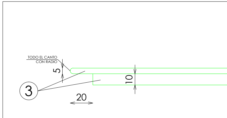
DETALLE TARIMA
