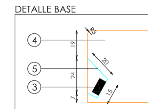
DETALLE BASE
