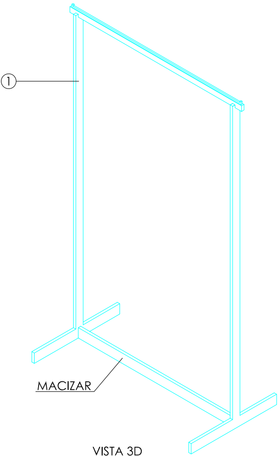
VISTA 3D
