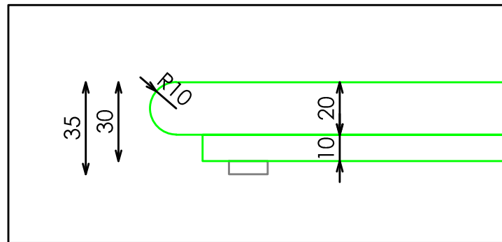
DETALLE TARIMA
