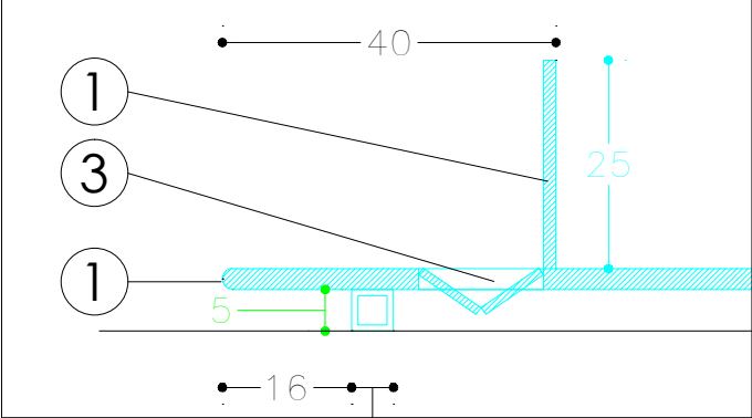
DETALLE BASE
