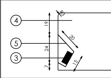
DETALLE BASE
