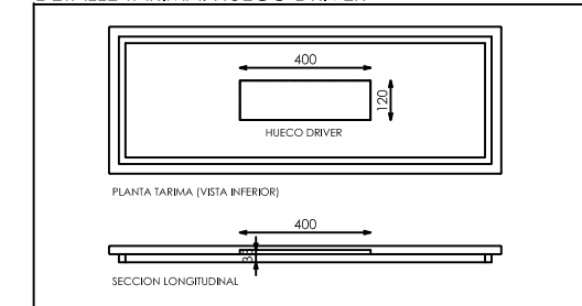
DETALLE BASE
