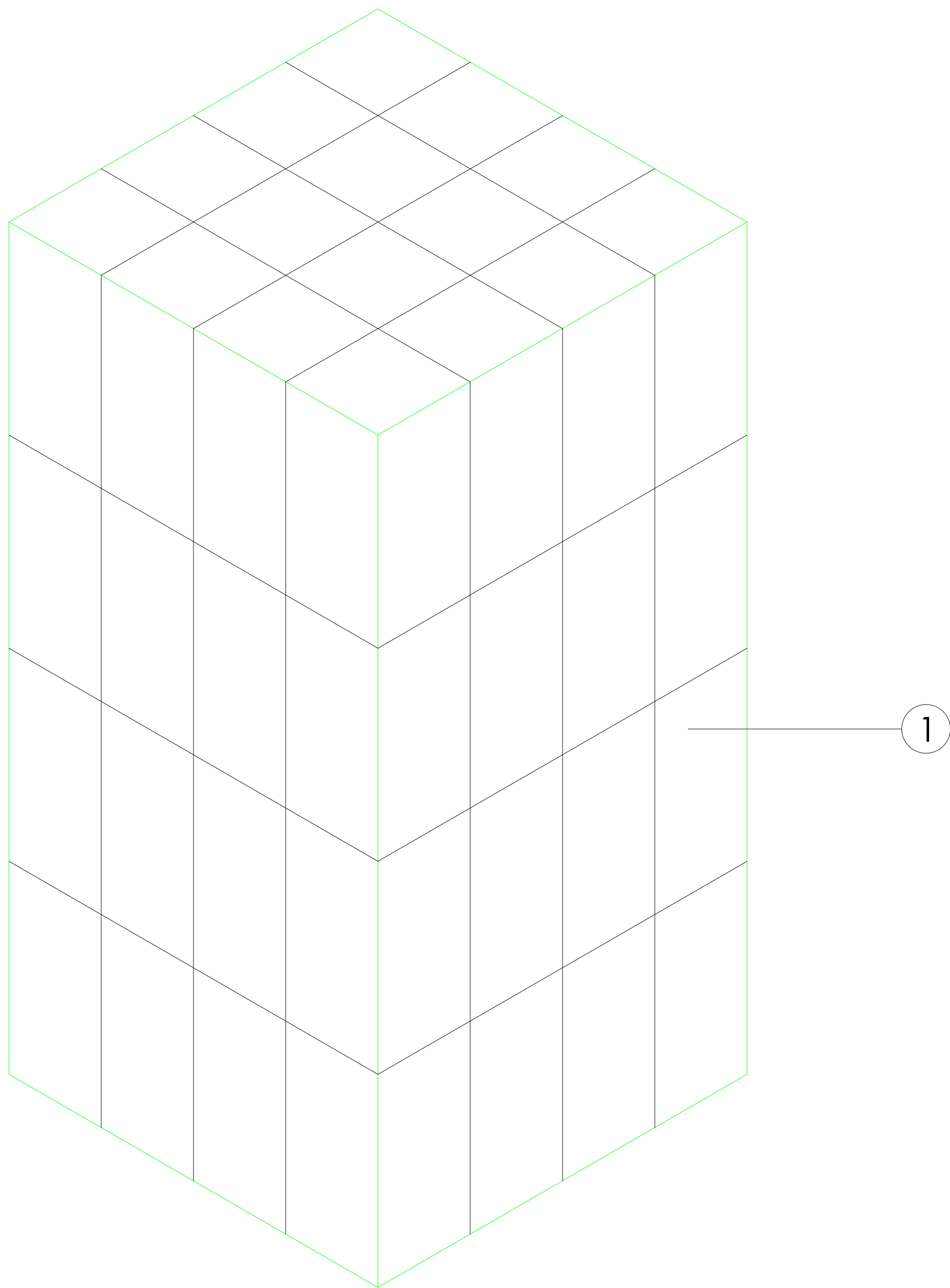
VISTA 3D
